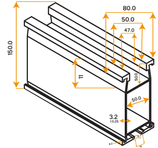
Aluminum Beam T150
