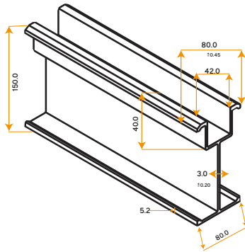
Aluminum Beam S150
