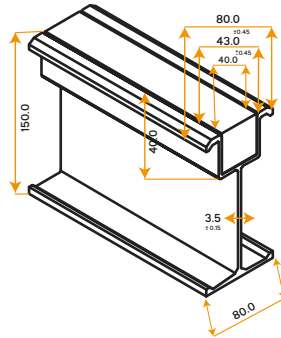
Aluminum Beam S150
