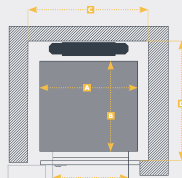
Rear-mounted system
