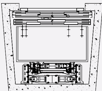
Special implementation of Silens Pro Compact® in an irregular and reduced shaft.
