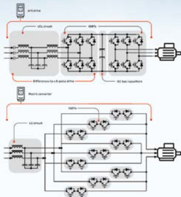
Low Harmonic VFDs
