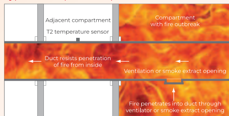
Type B Duct (fire inside)
